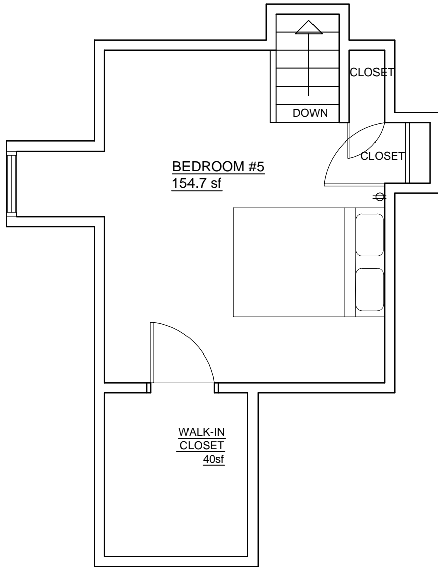
2nd FLOOR PLAN: 14 GUNN STREET 5 BEDROOM STUDENT RENTAL SCALE \frac{1}{4}" = 1'-0"
